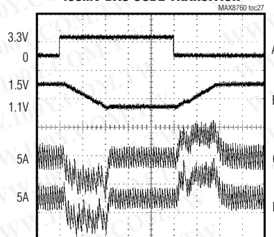
400mV DAC CODE TRANSITION
