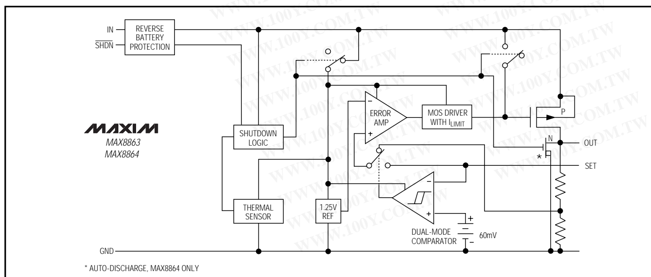
Figure 1. Functional Diagram
