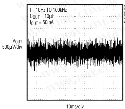
OUTPUT NOISE
