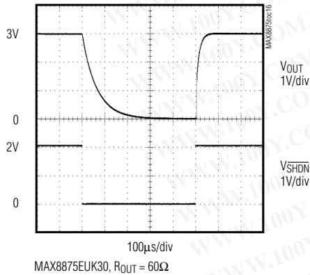
SHUTDOWN DELAY
