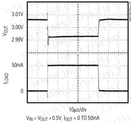
LOAD-TRANSIENT RESPONSE
