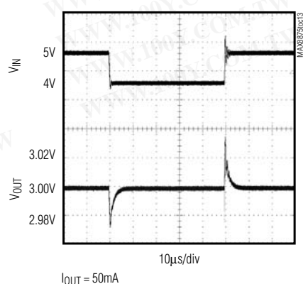
LINE-TRANSIENT RESPONSE
