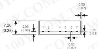
7 Pin SIL Package
