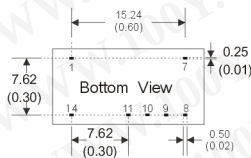
14 Pin DIL Package
