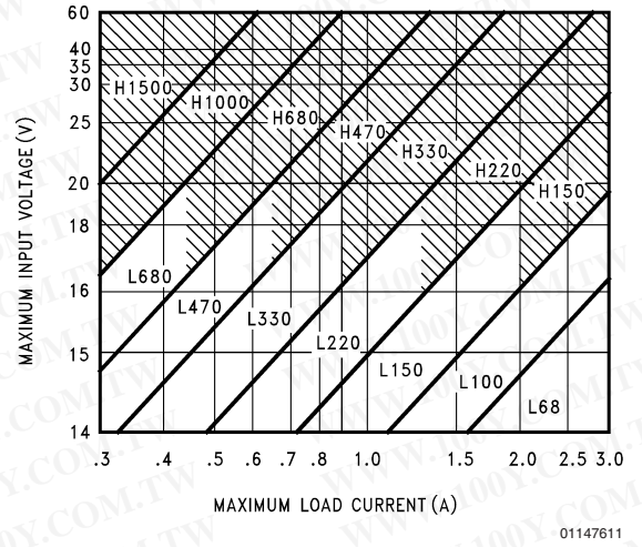
FIGURE 5. LM2576(HV)-12
