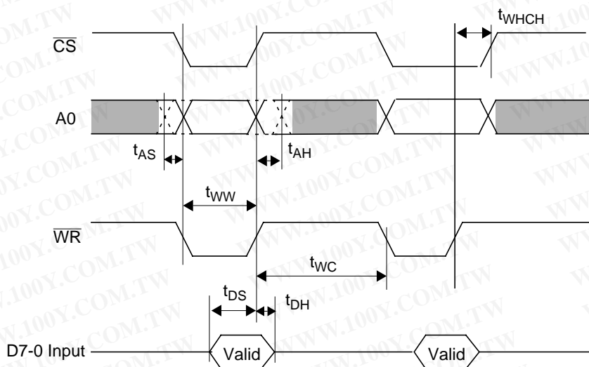
Figure 25. Non-Multiplexed Mode Write Timing (Consecutive Write Cycles Shown)
