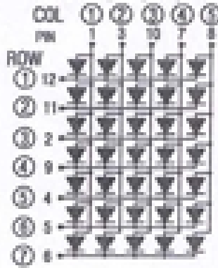
FIG.B N0757RS / G / O / E / Y N0757SY / SF / FS / PG
