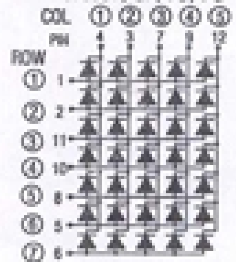
FIG.C N0756RS / G / O / E / Y N0756SY / SF / FS / PG
