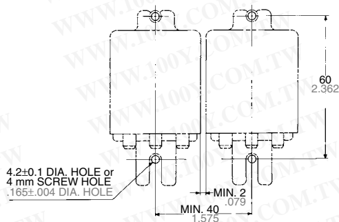
Mounting dimension
