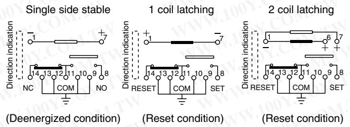
Schematic (Bottom view)
