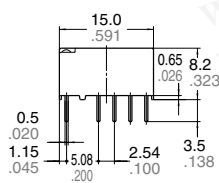
2 coil latching
