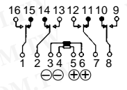
Schematic (Top view)
