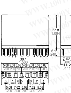
(NC4ED-L2)
