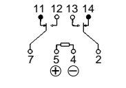
Deenergized position
