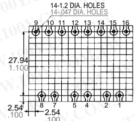
PC board pattern (Copper-side view)
