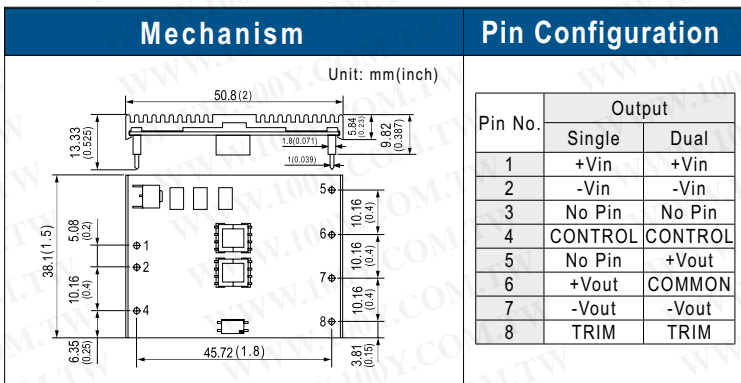
2" x 1.5" x 0.387"
