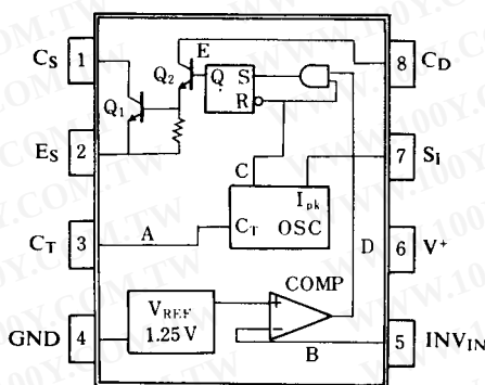
Fig. 1 Block Diagram
