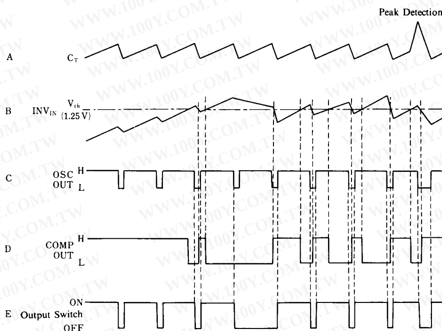
Fig. 2 Timing Chart
