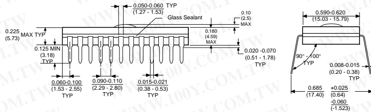
Dual-In-Line Package (Q) Order Number NMC27C64Q Package Number J28AQ
