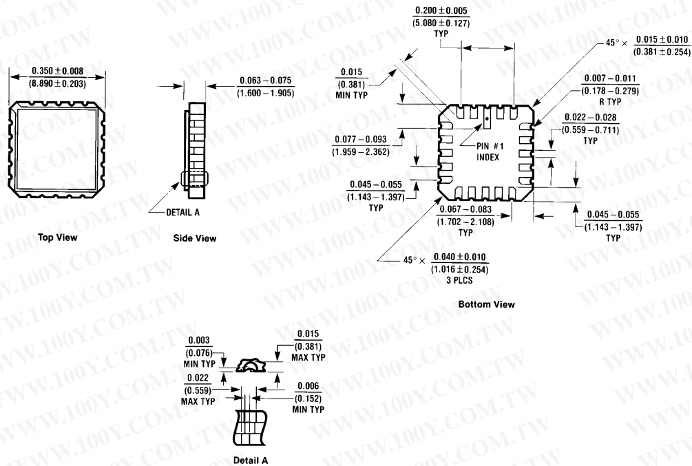
Ceramic Leadless Chip Carrier Package (E) Order Number 54LS04MQB NS Package Number E20A
