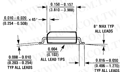
SOIC Package NS Package Number M08A
