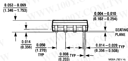
SOIC Package NS Package Number M08A
