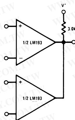
ORing the Outputs
