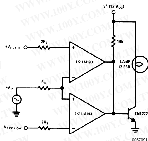
Limit Comparator
