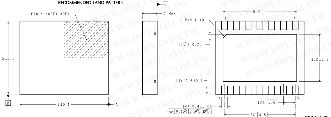
14-Lead LLP Package NS Package Number SRC14A
