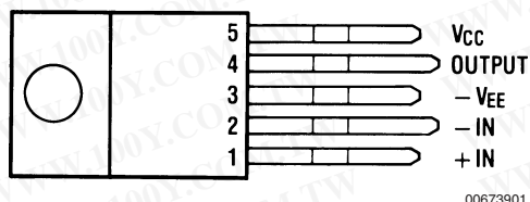
TO-220 Power Package (T)
