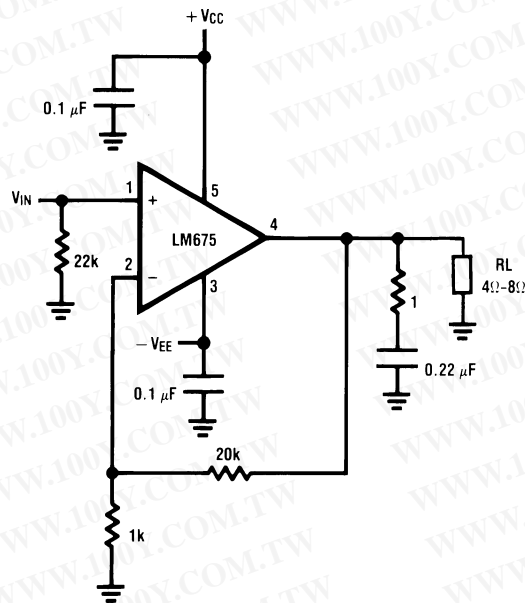
Non-Inverting Amplifier
