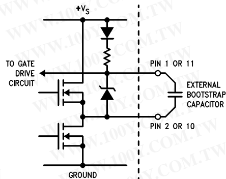
FIGURE 2. Bootstrap Circuitry
