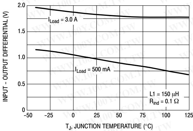
Figure 4. Dropout Voltage
