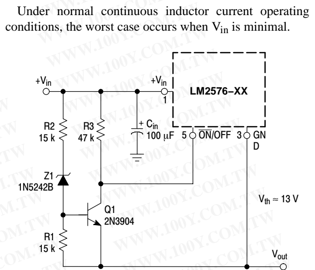
Figure 33. Undervoltage Lockout Circuit for Buck-Boost Converter
