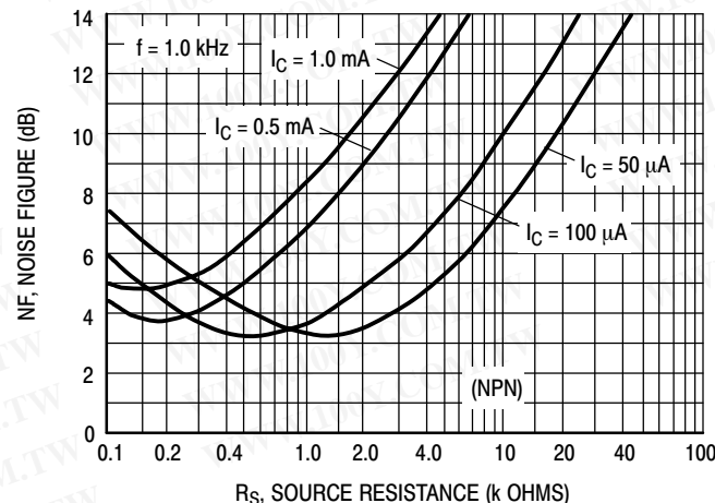
Figure 10. Noise Figure
