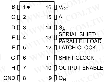
Figure 2. Pin Assignment
