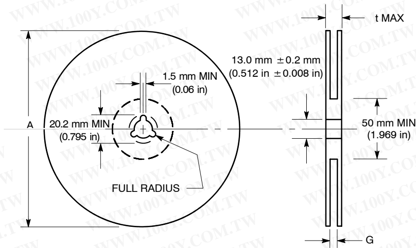
Figure 9. Reel Dimensions
