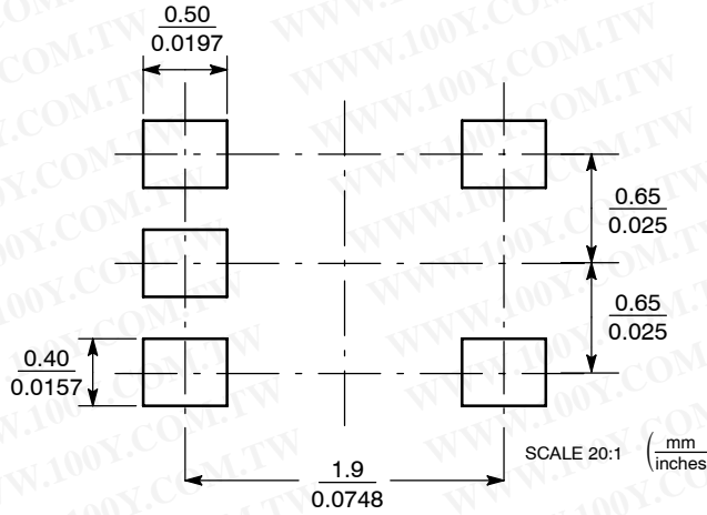
Figure 11. SC-88A/SC70-5/SOT-353
