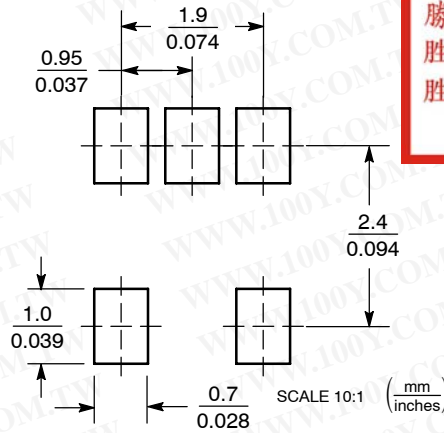
Figure 12. THIN SOT23-5/TSOP-5/SC59-5
