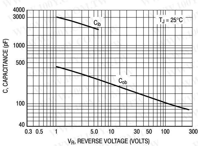
Figure 2. Capacitances
