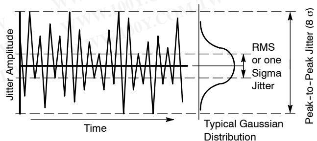
Figure 11. Peak-to-Peak Jitter
