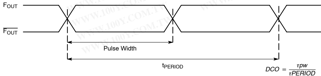
Figure 17. Output Duty Cycle
