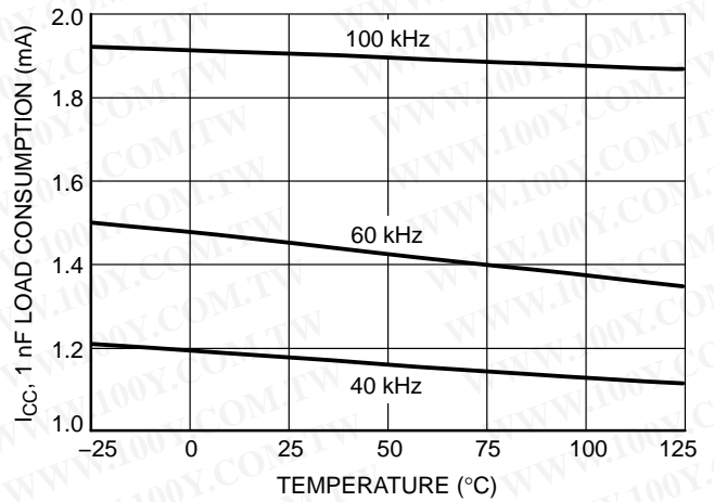
Figure 6. I C Consumption (Loaded by 1 nF) versus Temperature
