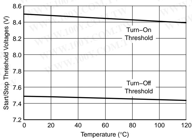
Figure 8. Undervoltage Lockout Thresholds vs. Temperature
