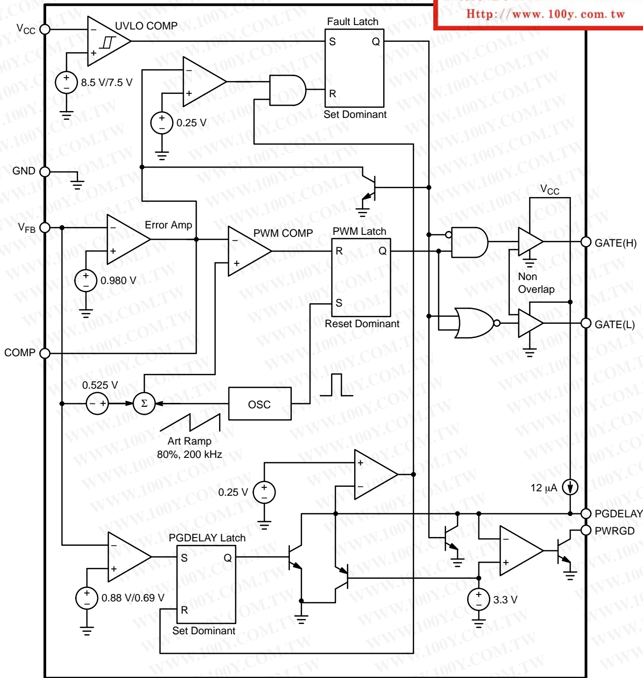
Figure 2. Block Diagram
