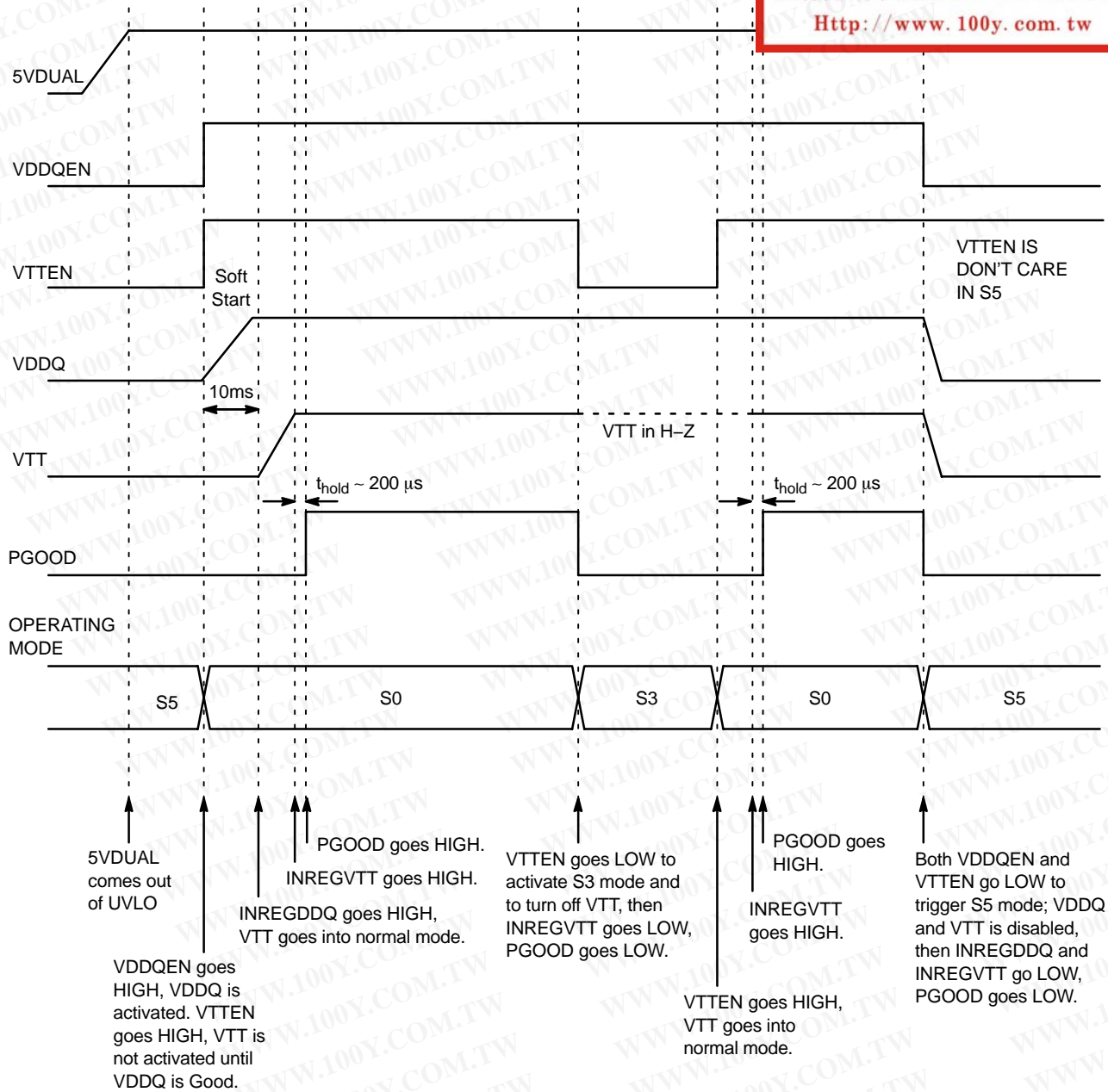
Figure 3. Powerup and Powerdown Timing Diagram
