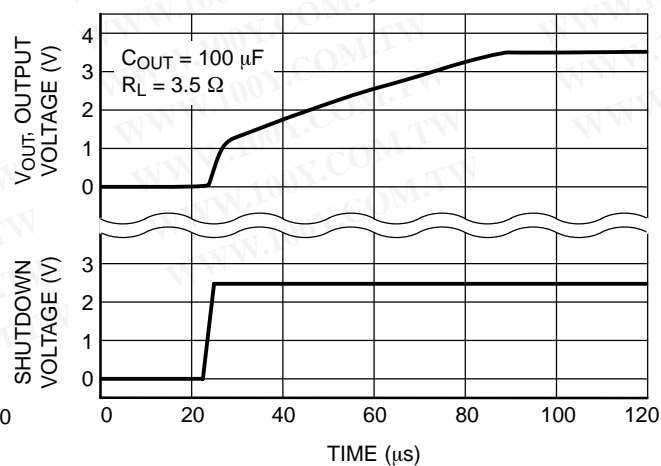
Figure 8. Start-up Transient
