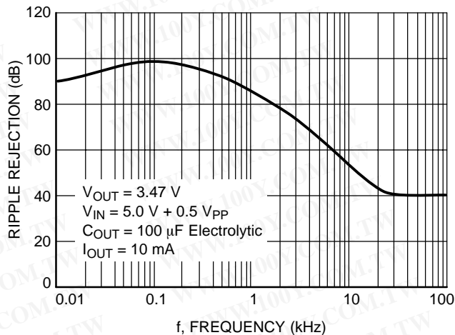
Figure 10. Ripple Rejection
