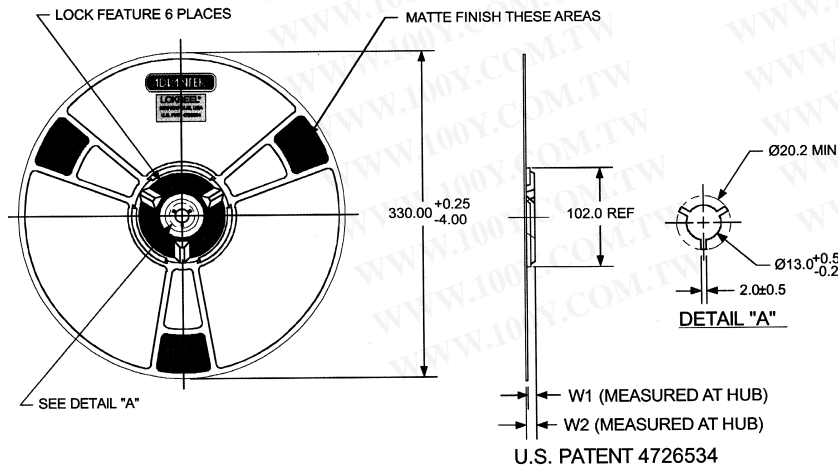
Figure 13. Reel Dimensions
