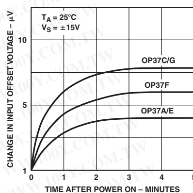
TPC 12. Warm Up Offset Voltage Drift
