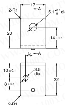
Y92E-SS05 (for M5 screw)
