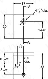
Y92E-SS04 (for M4 screw)
