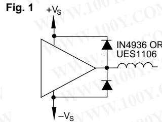
PROTECTION, INDUCTIVE LOAD
