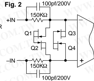
PROTECTION, OVERVOLTAGE
