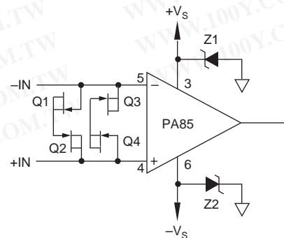
FIGURE 2. OVERVOLTAGE PROTECTION
