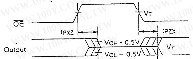
OE to Output Disable/Enable
