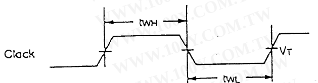
Clock Width
