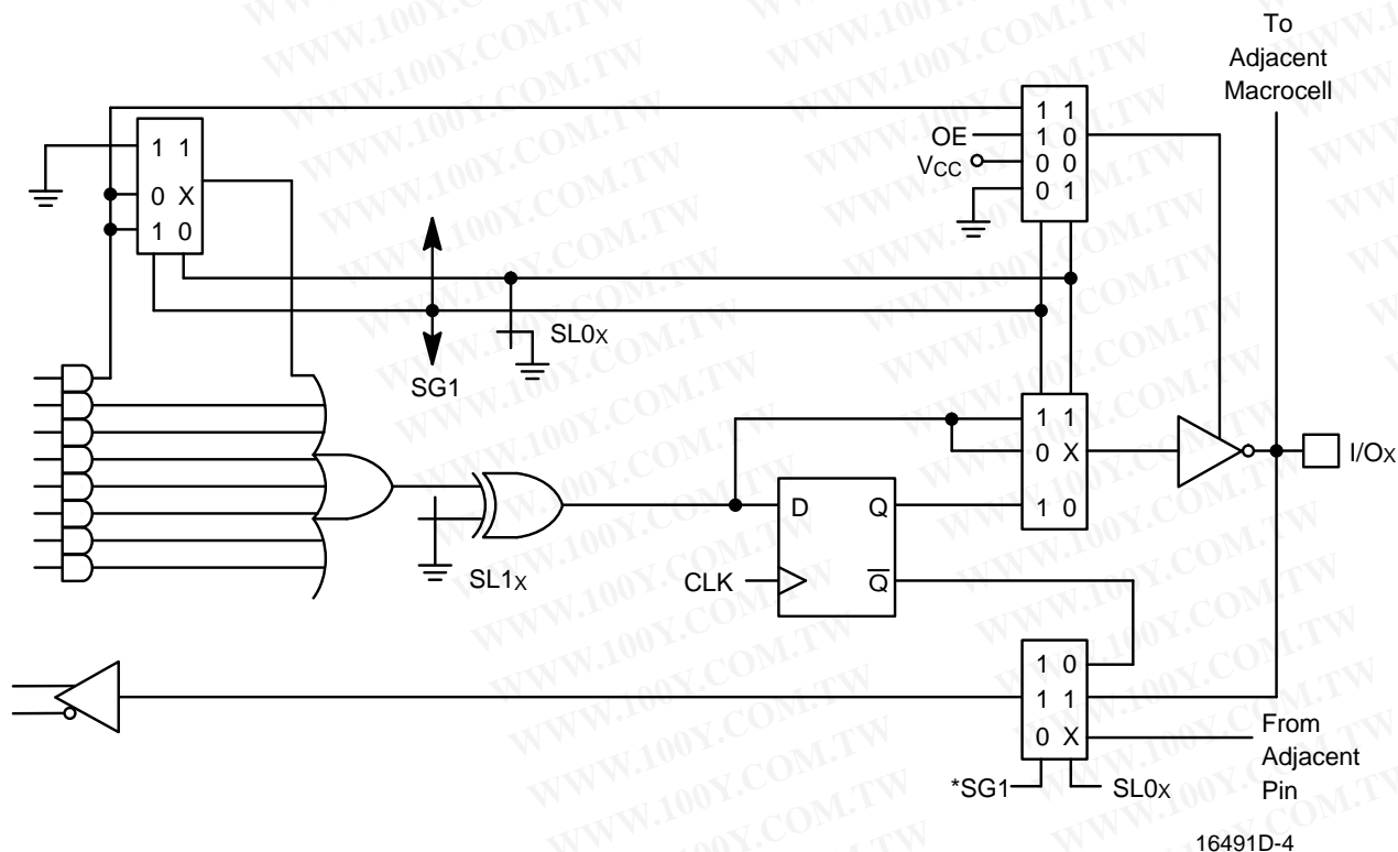
Figure 1. PALCE20V8 Macrocell
