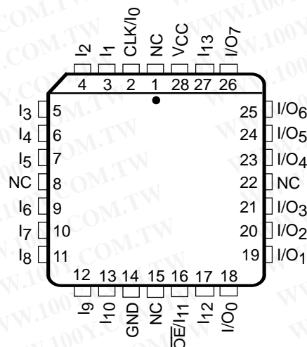
PLCC/LCC
