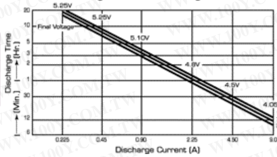
Discharge Time vs Discharge Current
