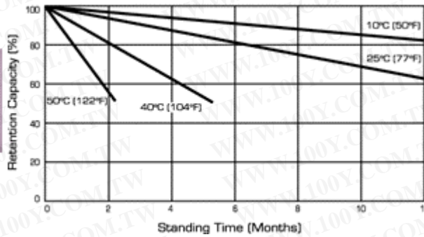
Shelf Life Characteristics
