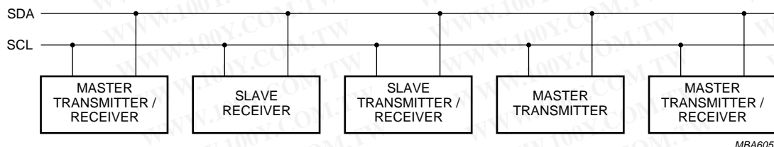
Fig.7 System configuration.
