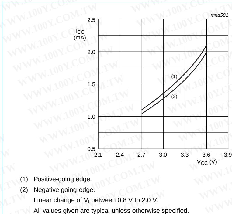
Fig 10. Average supply current as a function of supply voltage
