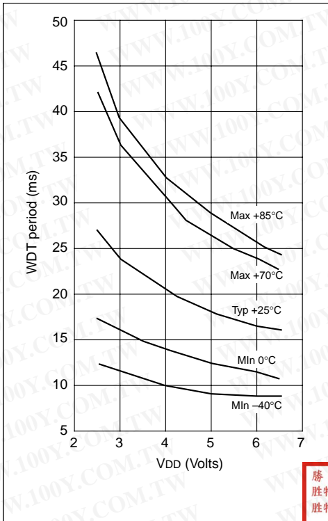
FIGURE 12-15: WDT TIMER TIME-OUT PERIOD vs. V DD
