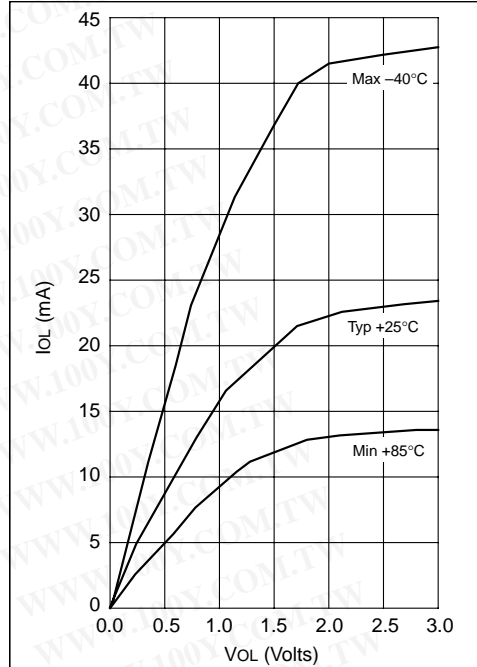
FIGURE 20-18: IOL vs. VOL, VDD = 5 V
