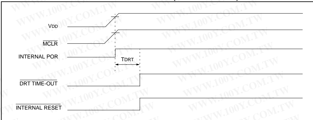
FIGURE 7-12: TIME-OUT SEQUENCE ON POWER-UP (MCLR TIED TO VDD): SLOW VDD RISE TIME
