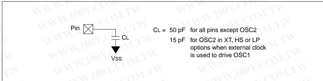
FIGURE 19-1: LOAD CONDITIONS - PIC16C54B/C54C/CR54B/CR54C/C55A/C56A/CR56A/C57C/CR57C/C58B/CR58B, PIC16CR5X
