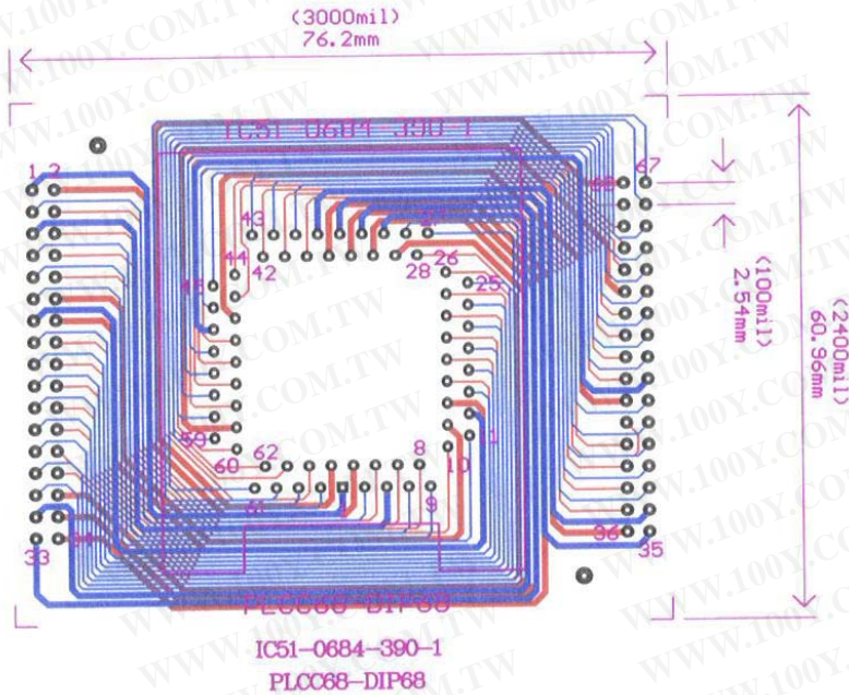
PCB Layout
