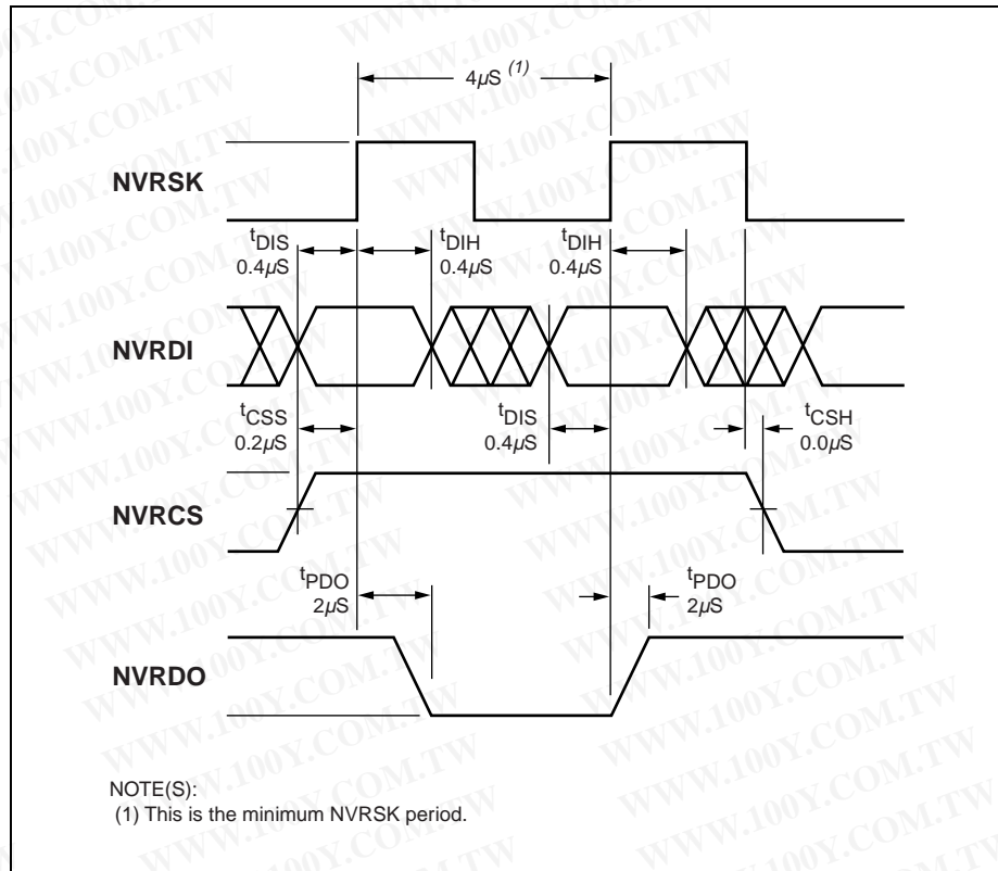
Figure 3-5. NVRAM Timing
