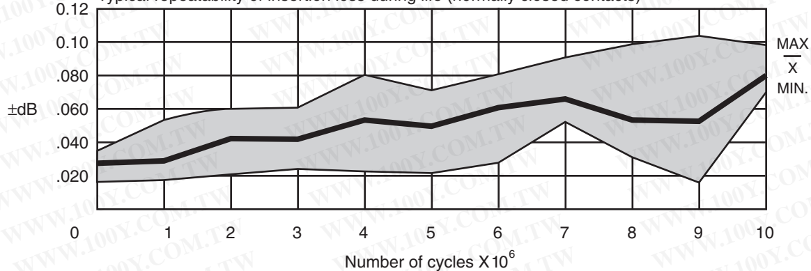
Typical repeatability of insertion loss during life (normally closed contacts)
