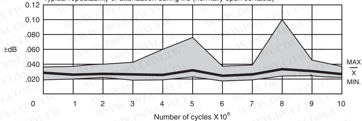
Typical repeatability of attenuation during life (normally open contacts)
