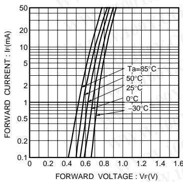
Fig.4 Forward characteristics
