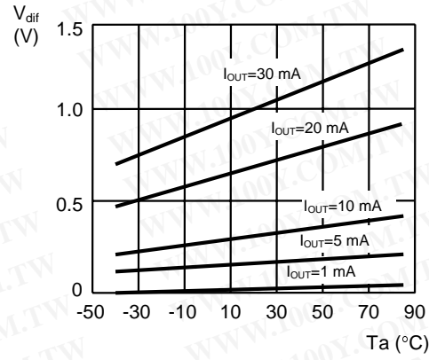
7.4 S-81225SG series
