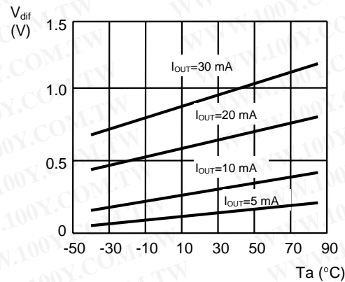
7.6 S-81235SG series
