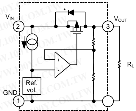
* Parasitic diode
