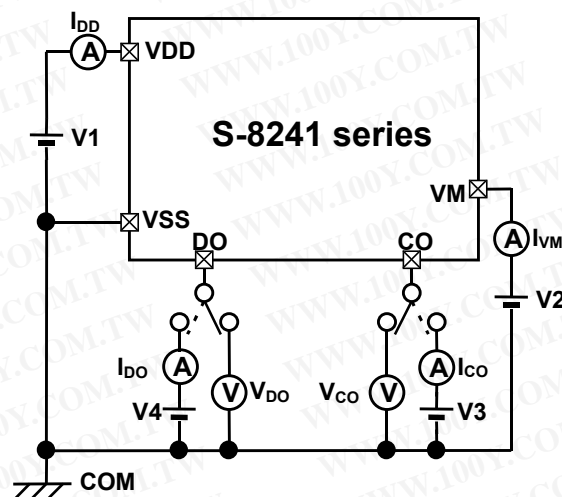
Measurement circuit 1
