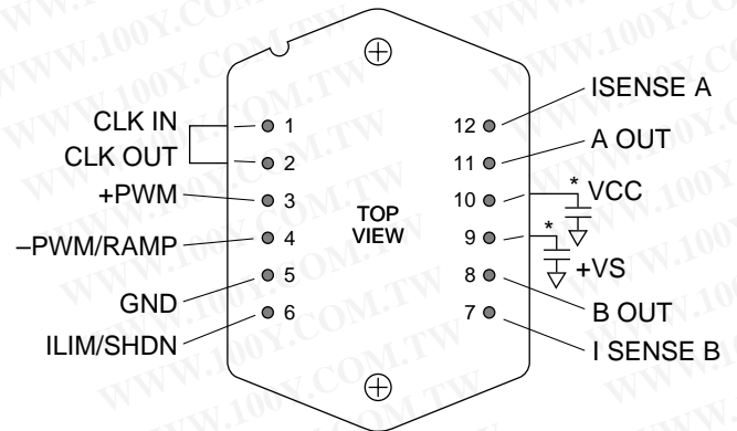
12-pin DIP PACKAGE STYLE DD
