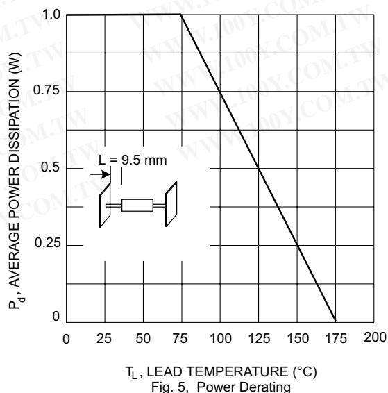
Fig. 5, Power Derating
