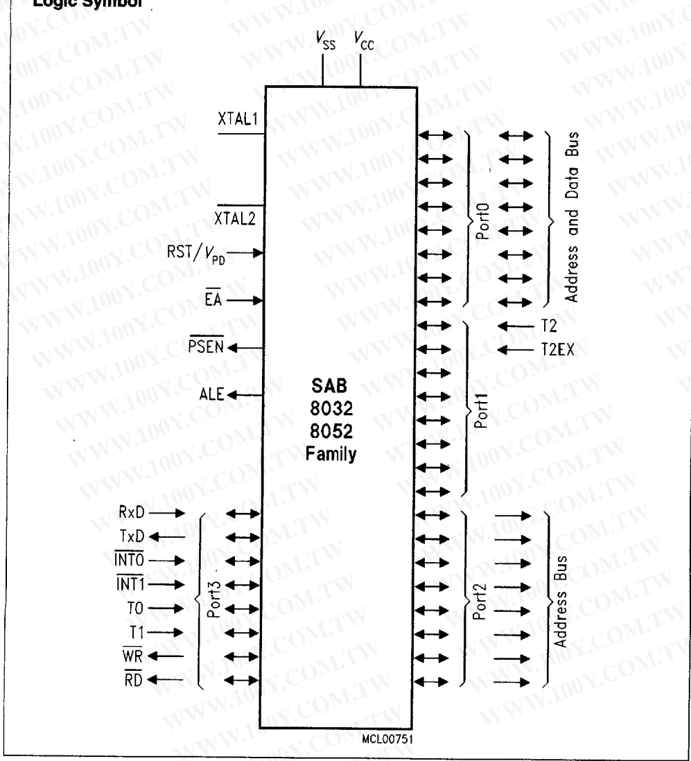
Figure 14 Logic Symbol
