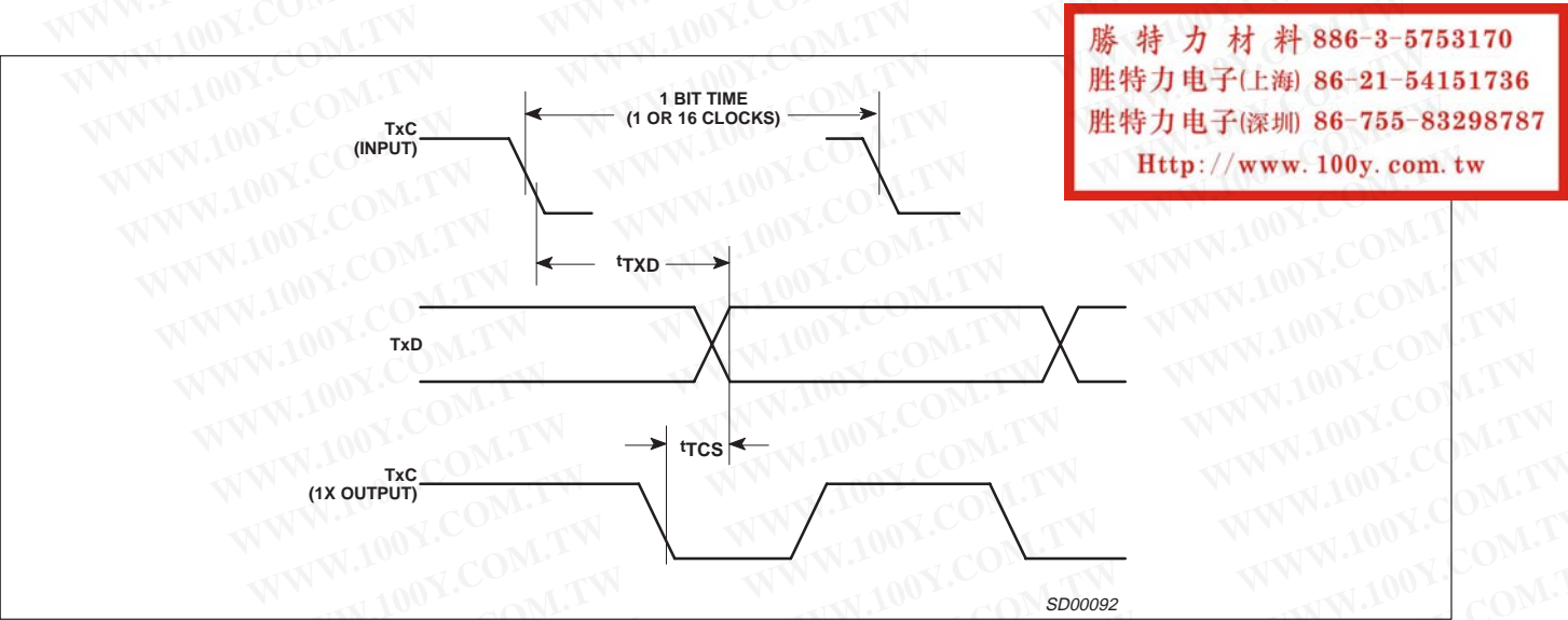
Figure 8. Transmit
