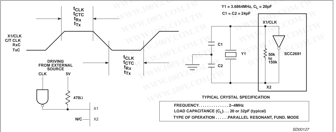
Figure 7. Clock Timing
