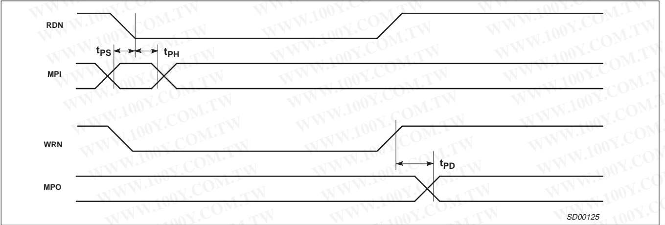
Figure 5. I/O Timing
