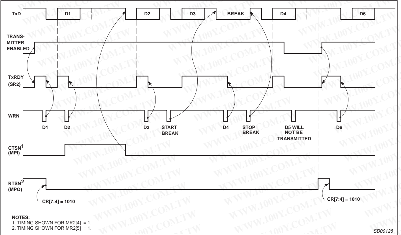
Figure 10. Transmitter Timing
